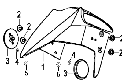
F14 FRONT FENDER
