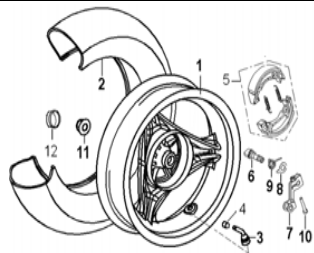
F09 REAR WHEEL
