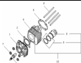
E01 CYLINDER HEAD ASSY
