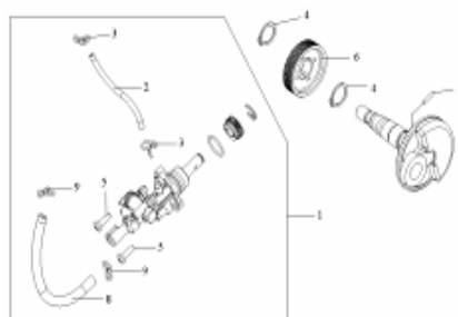
E10 CLUTCH SYSTEM ASSY PART TWO
