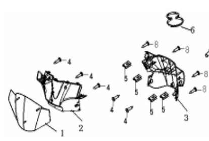
F15 HANDLE COVER
