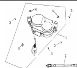
F20 SPEEDOMETER
