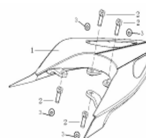
F15 HANDLE COVER
