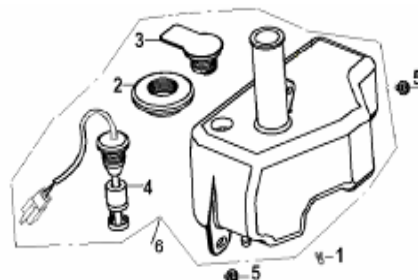
F13 OIL TANK
