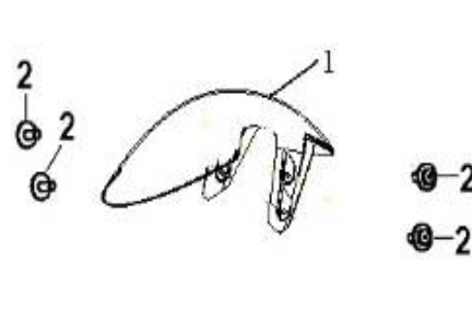
F14 FRONT FENDER
