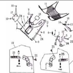
F16 FLOOR PANEL/FOOT REST
