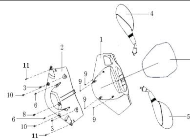
F14 HANDLE COVER
