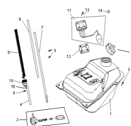
F08 FUEL TANK
