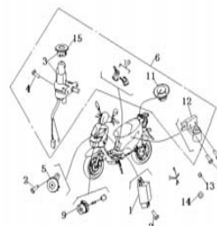
F23 ELECTRIC EQUIPMENT II
