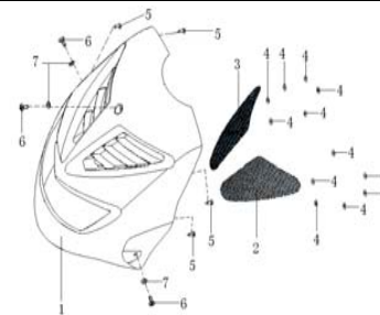
F15 FRONT COVER
