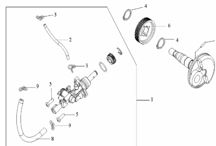
E10 CLUTCH SYSTEM ASSY PART TWO
