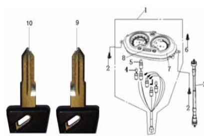
F23 ELECTRIC EQUIPMENT II
